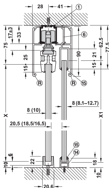
Ceiling installation with running track and clip panel 90 mm including fixed component. Sealing profile on one side for glass thickness 10 mm and wet sealing for glass thicknesses 8 – 12.7 mm.
