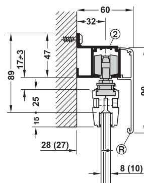
Wall mounting with running track and clip panel 90 mm
