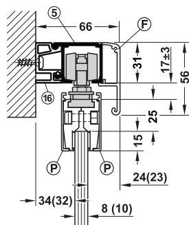
Wall mounting with running track and clip panel 56 mm, and clip panel on glass clamp shoe
