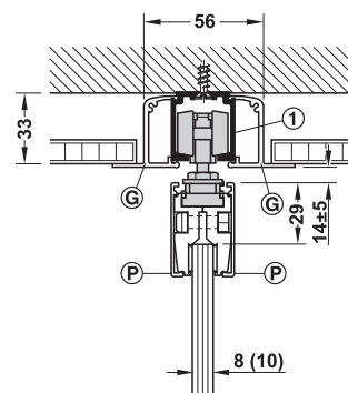
Ceiling installation with running track and 2 x clip panel for integration into suspended ceilings
