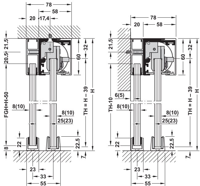
Ceiling installation and wall mounting
