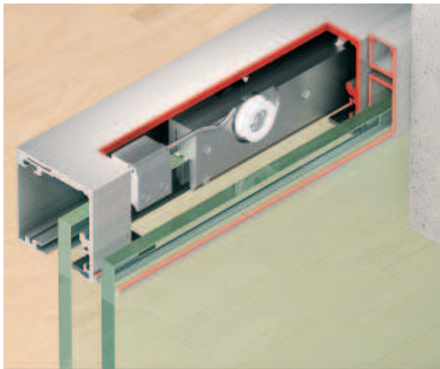
Ceiling installation and wall mounting
